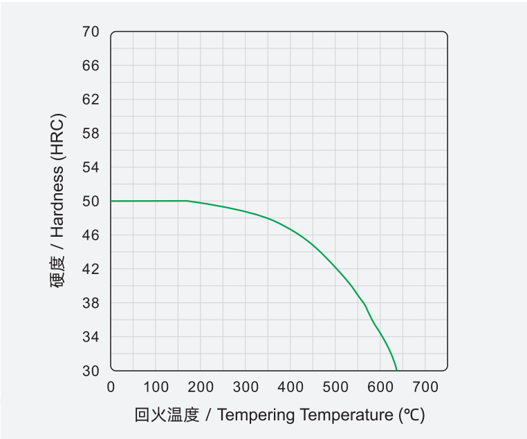
回火图（试样尺寸：Ø25 × 50mm；油淬温度：880℃） Tempering Curve (Sample dimension: Ø25x50mm; Quenched at 880℃ by Oil)
